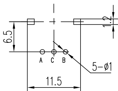
P.C.B MOUNTING HOLE DETAIL
